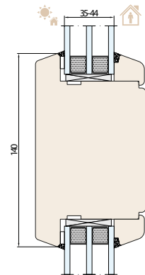
NATURO 80 SYSTEEM structurele roede 140 mm
