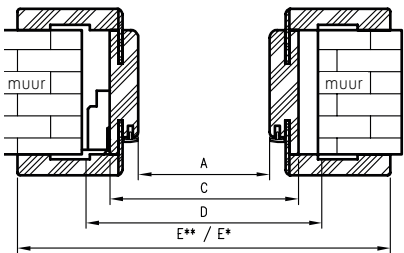
Horizontale doorsnede OR/ORC
