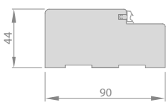
Vast frame
