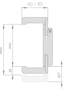
deurframeband 6/8 cm
